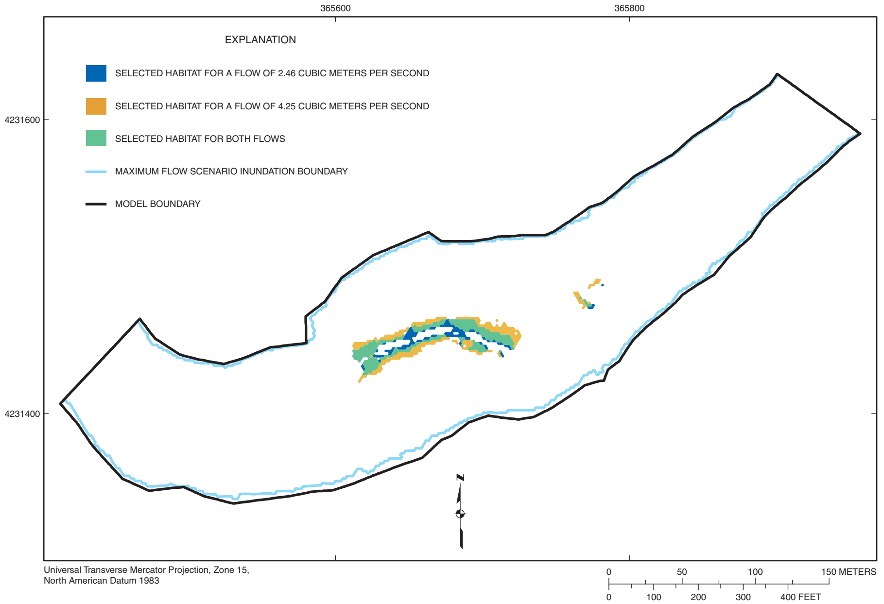
Figure 4-49. Selected habitat area distribution for habitat category 14 (flathead catfish) at flows of 2.46 and 4.25 cubic meters per second at Marais des Cygnes River site MDC2.
